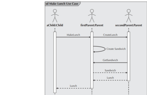
FIGURE 6-1 Example Sequence Diagram
