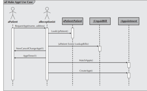
FIGURE 6-1 Example Sequence Diagram
