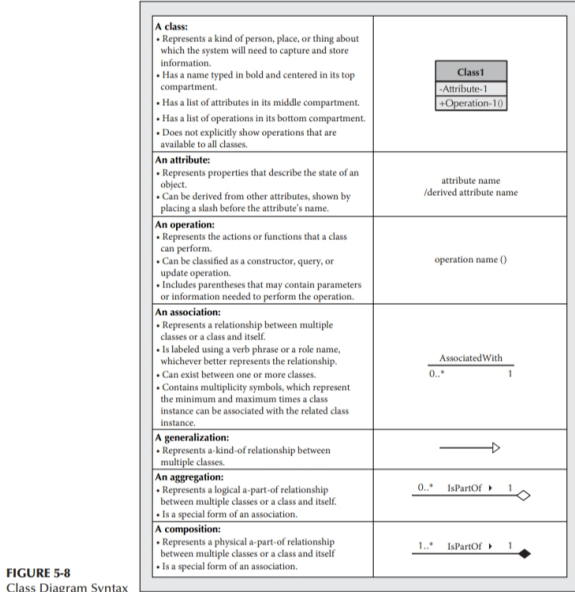
FIGURE 5-8 Class Diagram Syntax
