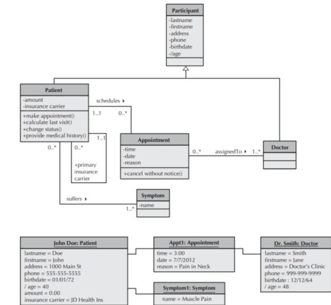
FIGURE 5-15 Sample Object Diagram
