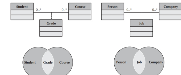
FIGURE 5-11 Sample Association Classes
