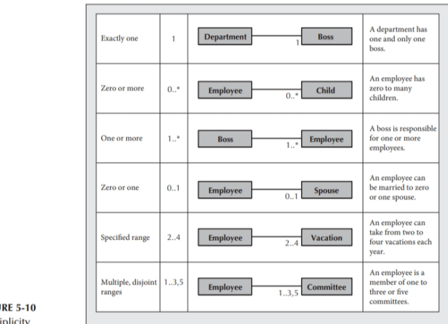
FIGURE 5-10 Multiplicity
